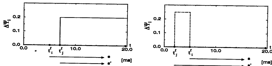
FIG. 3. Response kernel of the Mirrollo-Strogatz model. In the “phase” description (standard form I), the response kernel is a \theta function if s > s' (left) and vanishes for s < s' (right). In the “voltage” description, the response kernel is similar to the one-step integrate-and-fire model; see Fig. 2.
