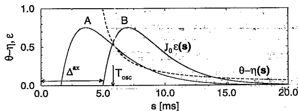
FIG. 4. Stability of a coherent oscillation. The intersection of the scaled response J_0\epsilon(s) (solid line) with the effective threshold (dashed line) \theta - \eta(s) yields the oscillation period T_{osc} . The oscillation is stable, if the slope of \epsilon(s) is positive at the intersection, as in case B (transmission delay \Delta^{ax} = 5 ms). It is unstable in case A ( \Delta^{ax} = 2 ms).
