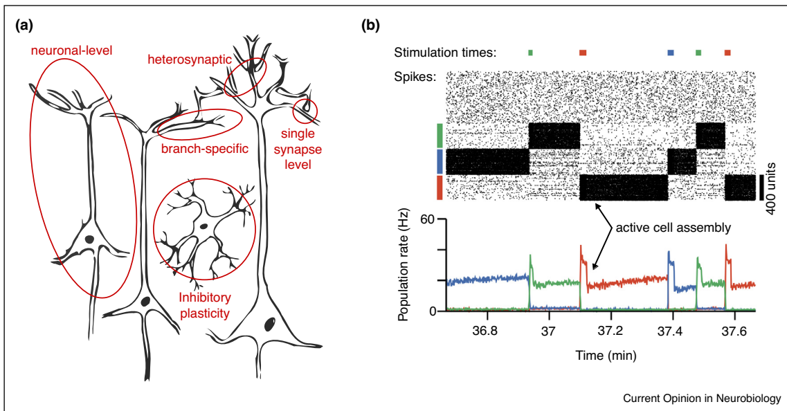
(a) Schematic representation of the many potential loci of rapid compensatory processes. (b) Example of a plastic network model displaying attractor dynamics in three distinct cell assemblies. Because these dynamics outlast the stimulus that triggers them they have been considered as neural substrate for working memory. The top panel shows a spike raster, whereas the bottom panel shows the population firing rates of the three cell assemblies. This particular model uses an augmented triplet STDP learning rule (cf. Figure 3) in which heterosynaptic plasticity and single-synapse-level plasticity have been added as stabilizing RCPs. Moreover, this model relies on a slow form of inhibitory plasticity which normalizes the overall network activity and ensures that cell assemblies do not grow indefinitely over time by recruiting additional neurons. This provides a proof of principle that a biologically inspired learning rule can indeed be stabilized by a sensible combination of RCPs, whereas the same learning rule endowed with slow compensatory mechanisms leads to run-away dynamics (cf. Figure 3b–d). Figure adapted from Zenke et al. [73].
